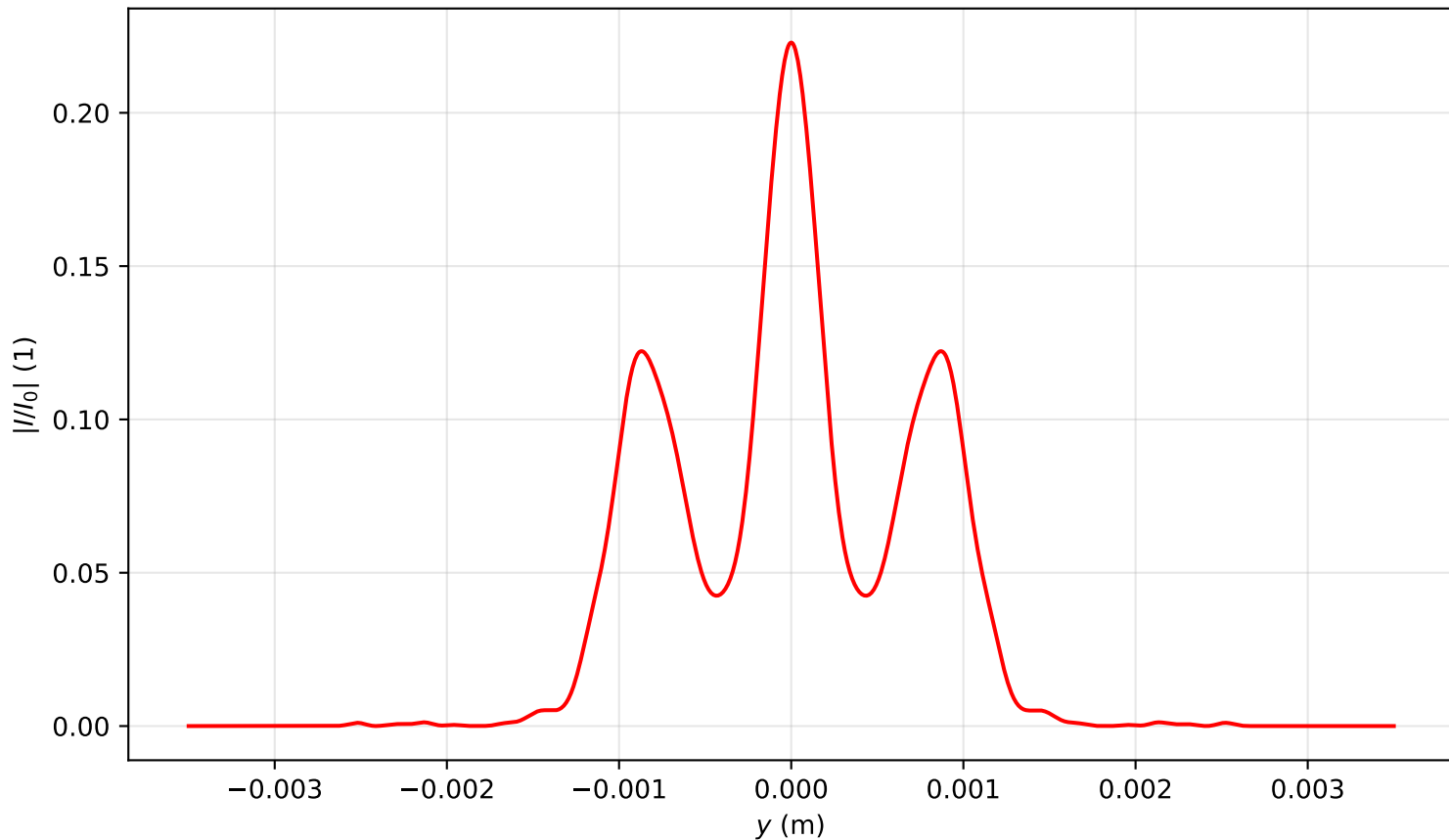
Intensity profile I(x=0, y, z=2.149)/I_0 , P_{in}=7.5P_{cr} , artificial time
